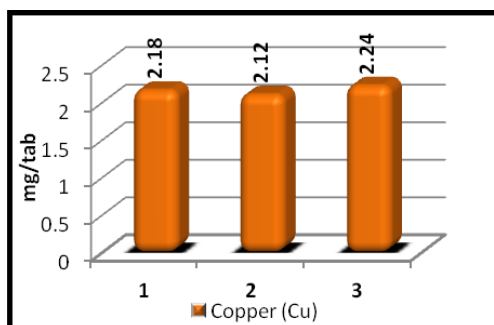
Graphical Representation of Copper Content in Sootikabharan Rasa (Batch to Batch Consistency) by ICP-OES
