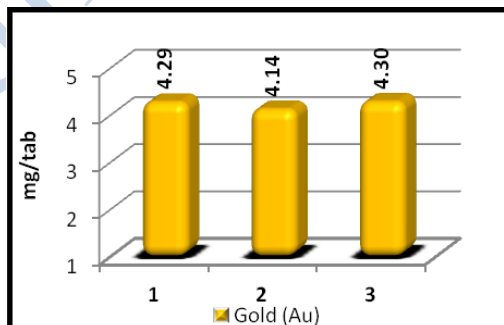
Graphical Representation of Gold Content in Sootikabharan Rasa (Batch to Batch Consistency) by ICP-OES
